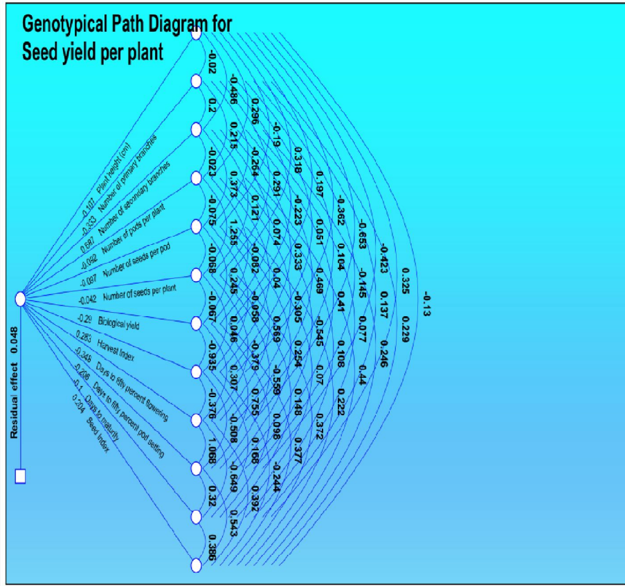
Fig 3: GENOTYPIC PATH DIAGRAM
