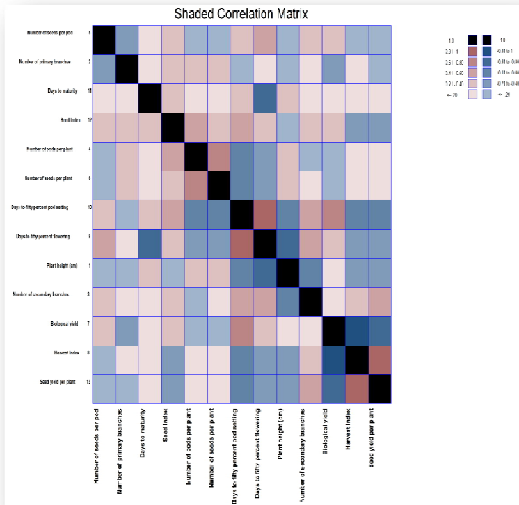
Fig 1: Genotypic Correlation Matrix
