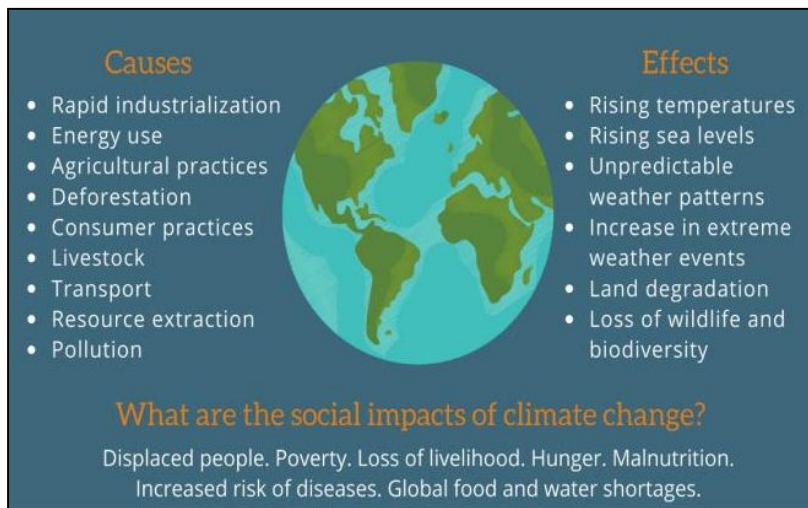
Fig 2: Causes and effect of climate change
