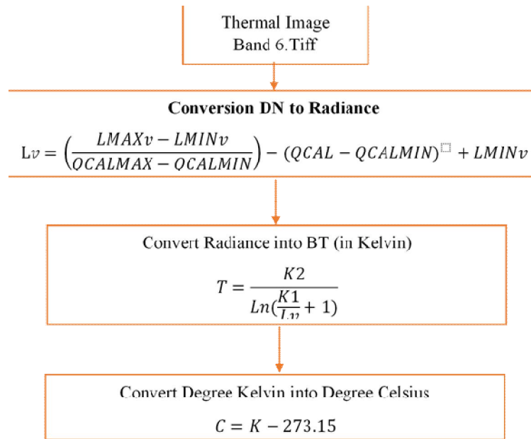
Figure 2: Formulas for estimating land surface temperature (LST)
