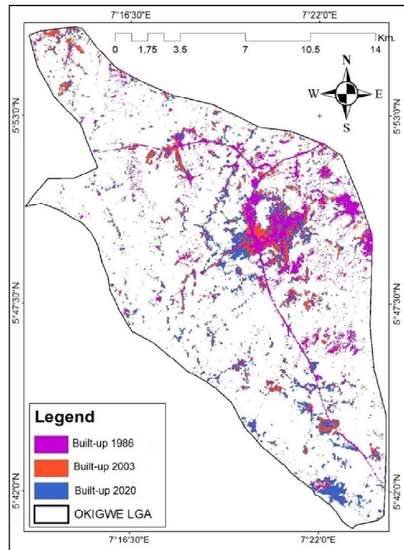
Figure 7: LULC Built-up Change Detection Map of Okigwe 1986-2003-2020
