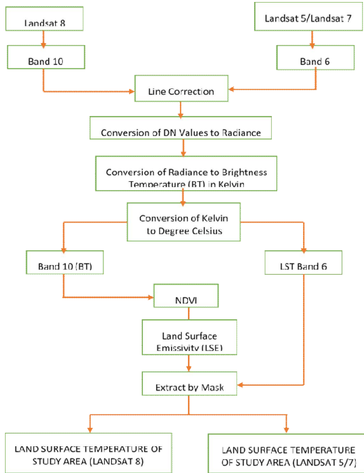
Figure 3: Land Surface Temperature Analysis Flow [28]
