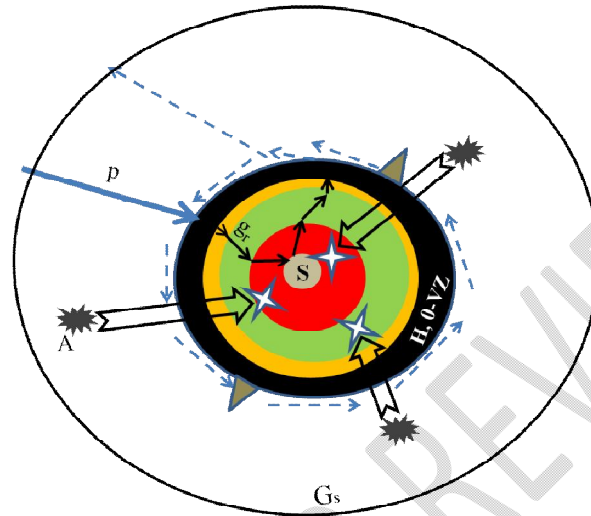
Figure 6. Schematic structure of black hole shows decreasing gravity layers until singularity center (S). Captured photon input (p) are transmitted as graviton ( g_r ) inside black hole until singularity, and reflected to reach horizon (H, 0-velocity zone). Asteroids (A) falling into black hole provoked phase transformations (blue stars), resulting in kinetic energy and related volcanic eruptions (grey triangles). Energy released and rotation allow possible phase particle changes and propagation around and outside the gravitosphere ( G_s ) (dashed arrows).
