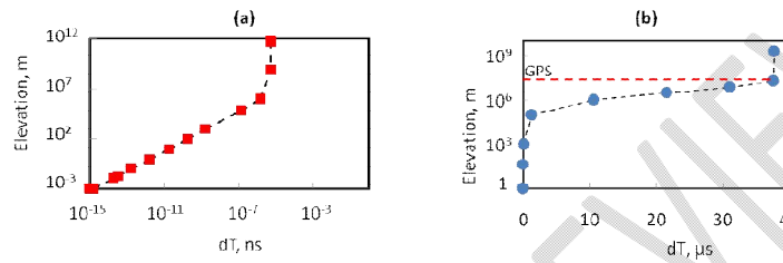
Figure 1. Time variations at increased elevation based on gravity changes and related velocity of photons (a), and satellites based GPS (b)
