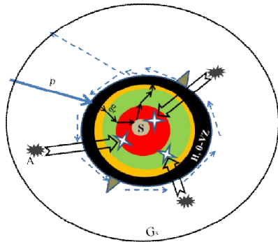
Figure 6. Schematic structure of black hole shows decreasing gravity layers until singularity center (S). Captured photon input (p) are transmitted as graviton (gr) inside black hole until singularity, and reflected to reach horizon (H, 0-velocity zone). Asteroide (A) failing into black hole provoked phase transformations (blue stars), resulting in kinetic energy and related volcanic eruptions (grey triangles). Energy released and rotation allow possible phase particle changes and propagation around and outside the gravitosphere (G) (dashed arrows).
