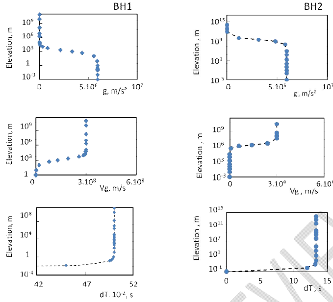
Figure 3. Variations of gravity, velocity and time variations versus elevation (in log) are determined for Black holes of 3km (BH1) and 8 \cdot 10^9 km (BH2) radius
