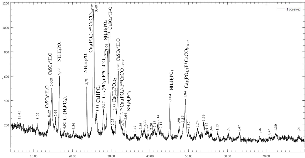
Figure 1. Radiograph of enriched superphosphate on base solid part of ammophosphate pulp.
