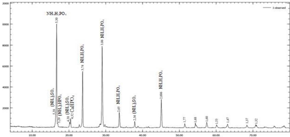
Figure 2. Radiograph of concentrated ammophosphate fertilizer based on liquid part of ammophosphate pulp.
