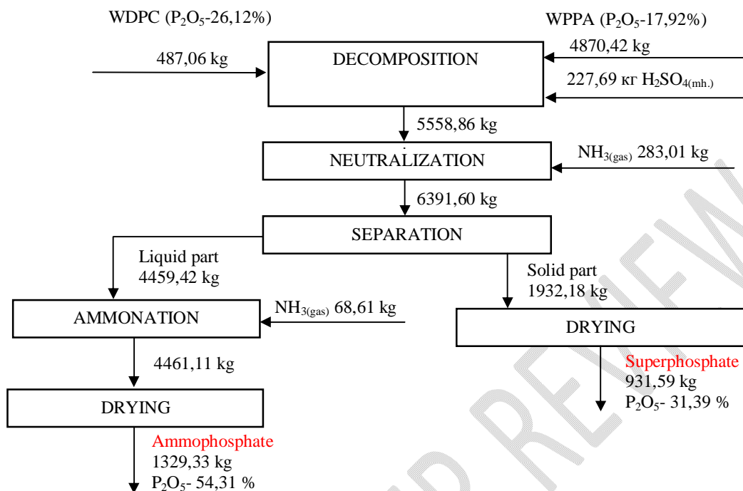
Fig. 3. The material balance of enriched superphosphate and concentrated ammophosphate in a single technological cycle.
