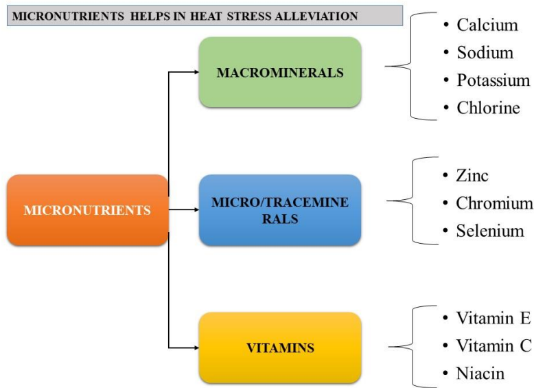
Fig. 2 Classification of important micronutrients helps in heat stress alleviation
