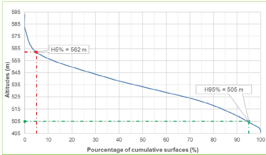
Figure 4: Hypsometric curve of Sokouraba watershed
