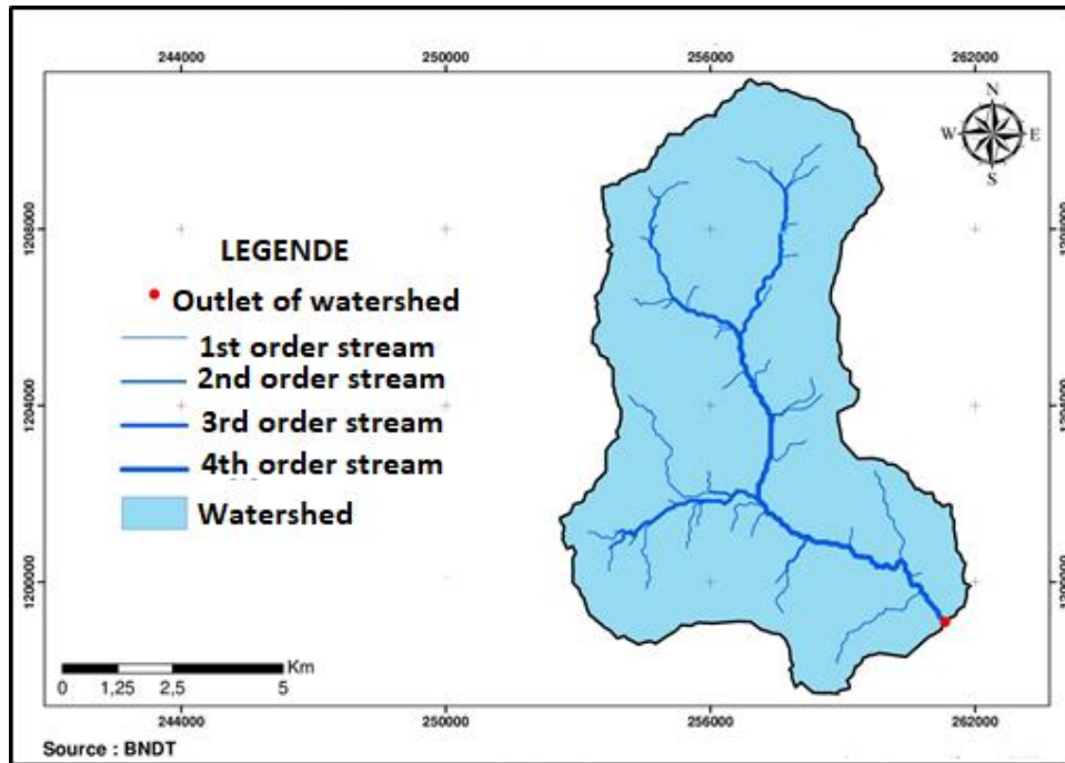
Figure 2: Sokouraba watershed and its hydrographic network
