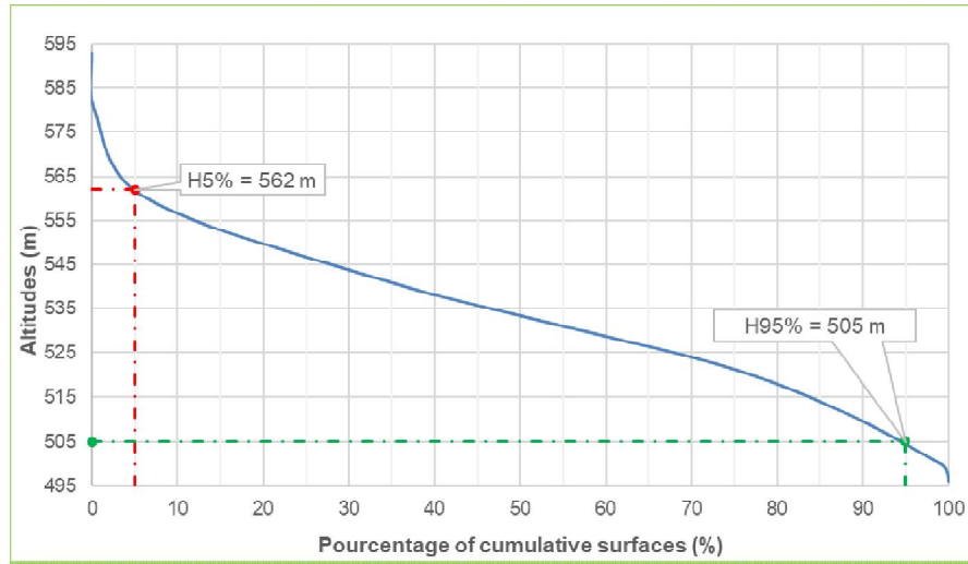
Figure 5: Hypsometric curve of Sokouraba watershed
