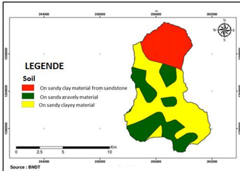
Figure 6: Soil map of Sokouraba watershed
