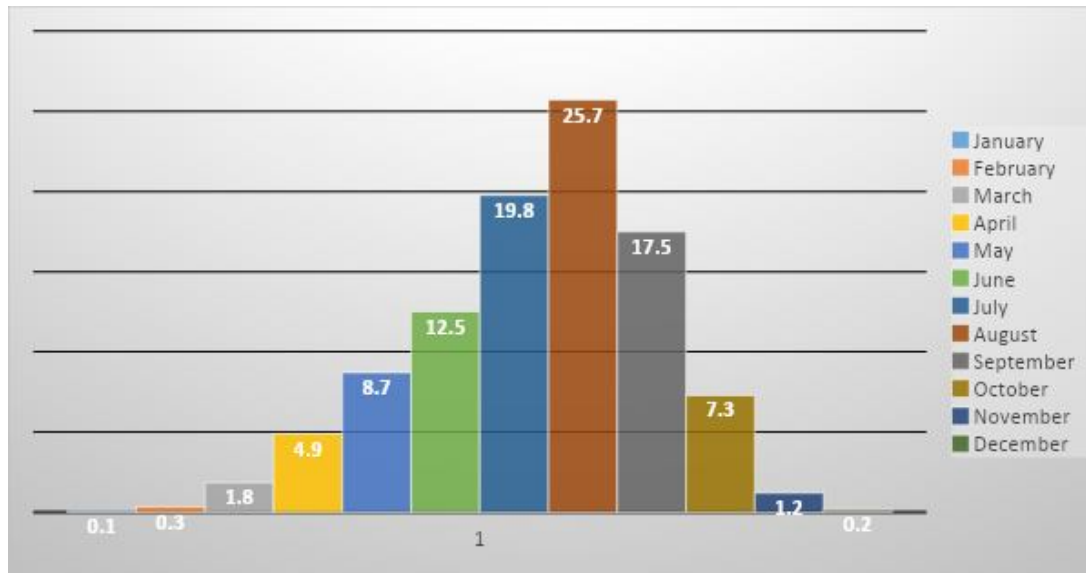
Figure 2: Histogram of annual rainfall for Orodara from 1960 to 2019
