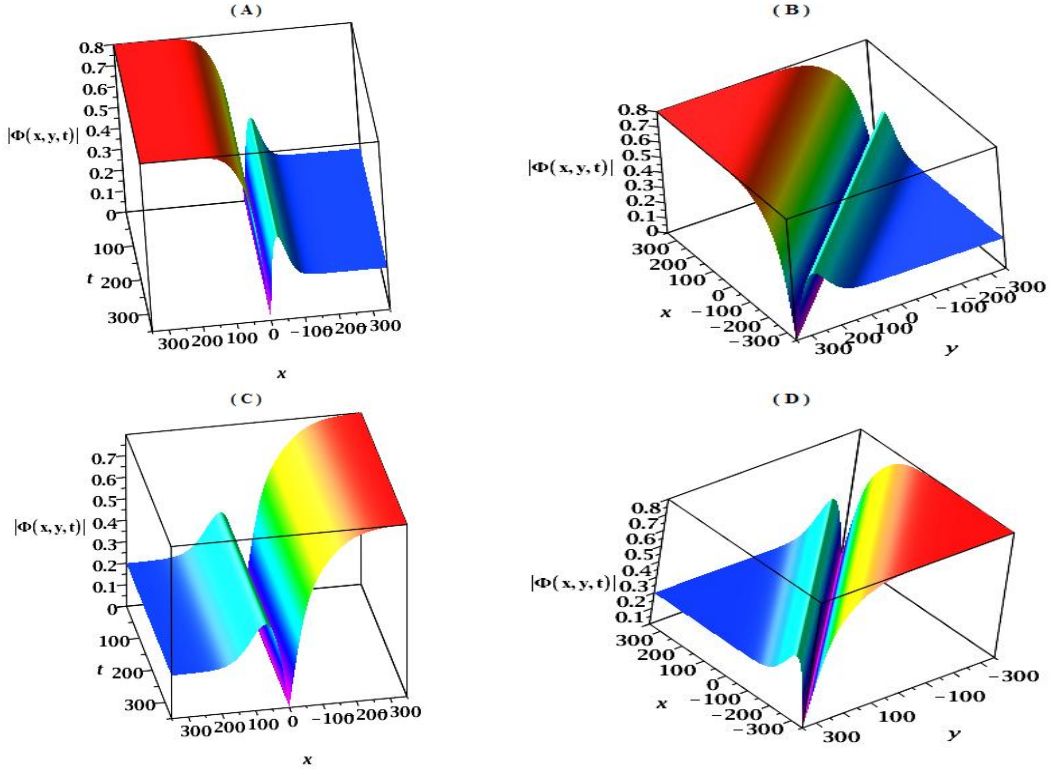
Figure 2: Graphical representation given by eq.(85). Top row, for \eta = 0.01; \gamma = 1; \nu = 0.0013; \alpha = -0.67; k = 0.1; s = 0.2; B_2 = \chi = 0.3; A_2 = 3B_2 = 3; B_1 = \frac{5}{3}B_2; \lambda = -1.720977806; G = 0.2813798713; \omega = 0.5861950181 : Antikink-Bright-Dark solitary waves: A) y = 0 ; B) t = 0 . Bottom row, for \eta = 0.01; \gamma = 1; \nu = 0.0013; \alpha = -0.67; k = 0.1; s = 0.2; B_2 = \chi = 0.3; A_2 = 3B_2; B_1 = -\frac{5}{3}B_2; \lambda = -1.720977806; G = 0.2813798713; \omega = 0.5861950181 : Kink-Bright-Dark solitary waves C) y = 0 ; D) t = 0 .
