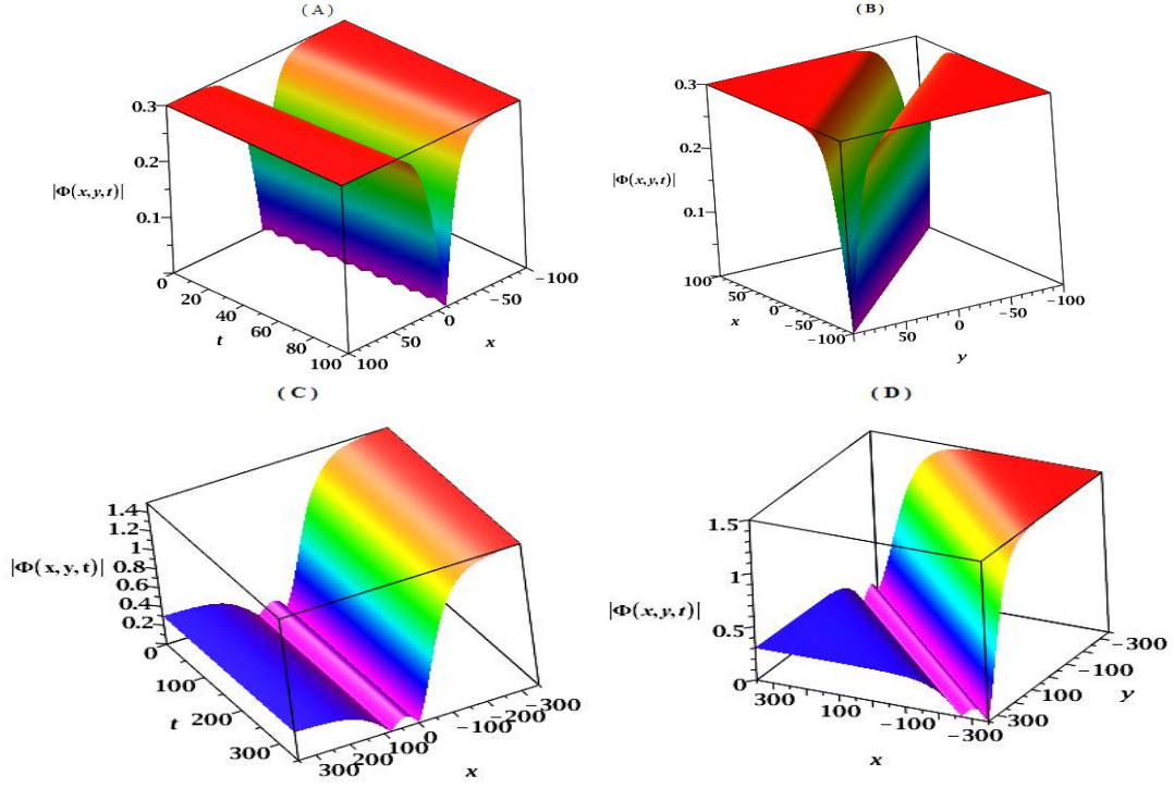
Figure 1: Graphical representations given by eq.(99) and (103). Top row, eq.(99) : for \eta = 0.05; B_1 = 0.3; \gamma = 0.03; k = 0.1; s = 0; \nu = -0.1; \alpha = -37; \lambda = -0.3333333333; G = 12; \omega = 0.08500000001 : Dark solitons with a sawtooth bottom: (A) : y = 0 (B) : t = 0 . Bottom row, eq.(103) : for \eta = 0.01; \lambda = 0.02; \alpha = -2.5; k = 0.1; s = 0.2; \gamma = -0.0015; \nu = 0.00026; B_1 = 0.6; B_2 = -1.5B_1 = -0.9; G = 0.30966; \omega = 0.42966 : Kink-Dark-Bright solitary waves C) y = 0 ; D) t = 0 .
