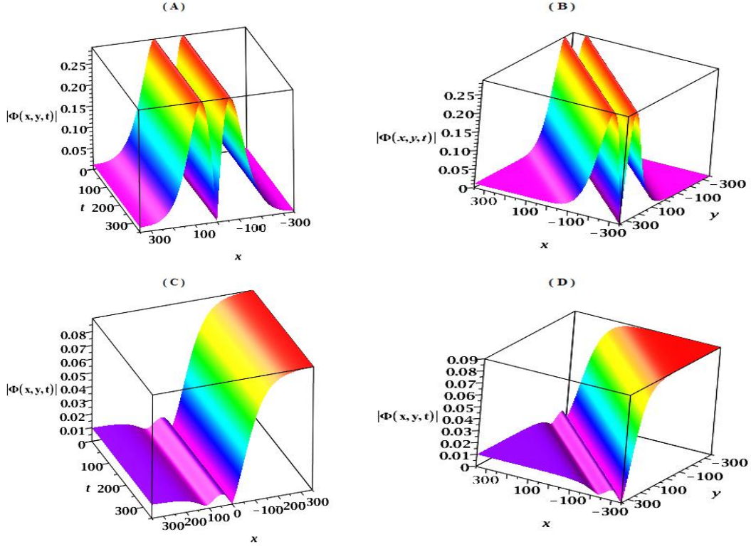
Figure 3: Graphical representation given by eq.(85). Top row , for \eta = 0.01; \gamma = 1; \nu = 0.0013; \alpha = -0.67; k = 0.1; s = 0.2; B_2 = \chi = 0.006; A_2 = 125B_2; B_1 = \frac{5}{6}B_2; \lambda = -0.9586430515; G = 0.1567381389; \omega = 1.048271134 : Double-Bright Dark solitary waves: A) y = 0 ; B) t = 0 . Bottom row , for \eta = 0.01; \gamma = 1; \nu = 0.0013; \alpha = -0.67; k = 0.1222; s = 0.2; B_2 = \chi = 0.05; A_2 = 0.16B_2; B_1 = -0.8B_2; \lambda = -0.5211797094; G = 0.02736193474; \omega = 1.923607548 : Kink-Dark-Bright solitary waves: C) y = 0 ; D) t = 0 .
