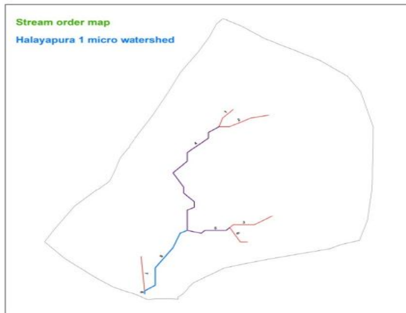
Fig.2 Stream order map of Halayapura micro-watershed
