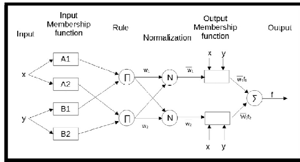
Figure 6 ANFIS Architecture
