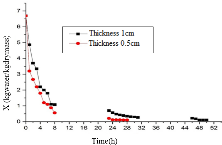
Figure 5: Variation of water content as a function of time and thickness
