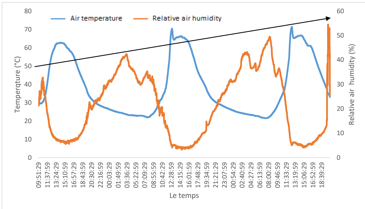
Figure 3: Changes in temperature and relative air humidity on the fourth rack
