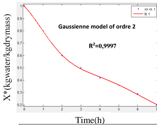
Figure 8 : fitting of the drying kinetics by the Gaussian of order 2
