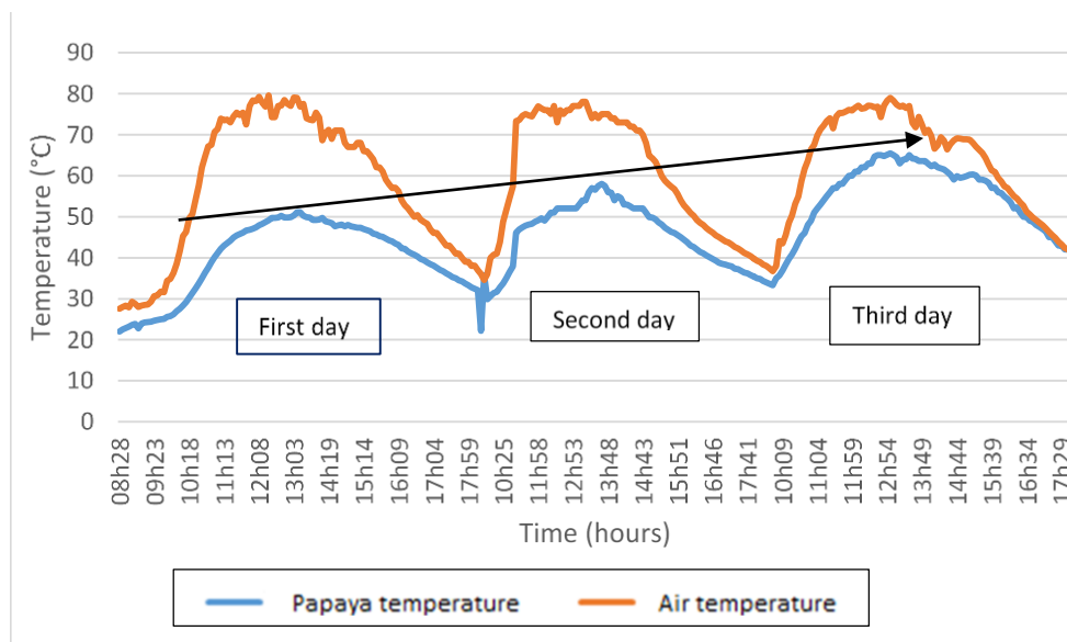
Figure 2: Changes in the temperature of the rack and that of the papaya during drying
