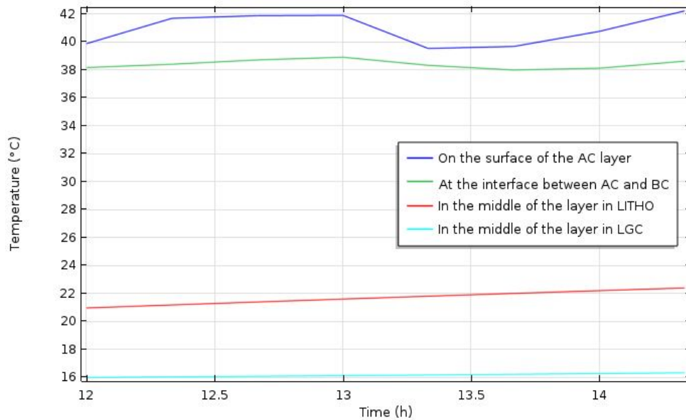
Fig. 7.c Evolution of the temperature in the different layers of the NR4 during the rainfall of maximum intensity of 53.6 mm/h.
