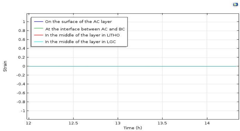
Fig. 9.d Temporal distribution of longitudinal deformations in the different layers of NR4 during a rainfall of maximum intensity of 99 mm/h.
