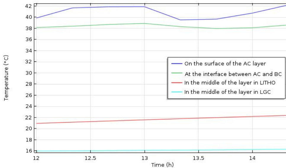
Fig. 7.d Evolution of the temperature in the different layers of the NR4 during the rainfall of maximum intensity of 53.6 mm/h.
