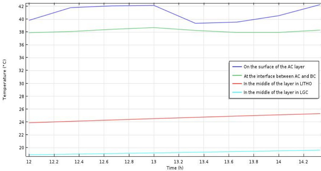
Temperature evolution in the different layers of NR2 during the maximum rainfall intensity of 99 mm/h.
