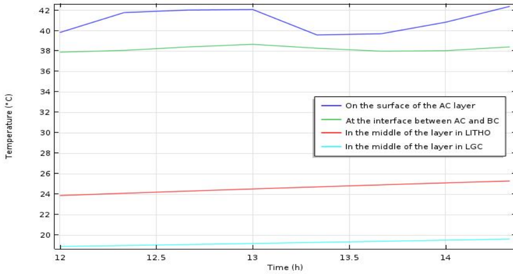
Evolution of the temperature in the different layers of the NR2 during the rainfall of maximum intensity of 53.6 mm/h.
