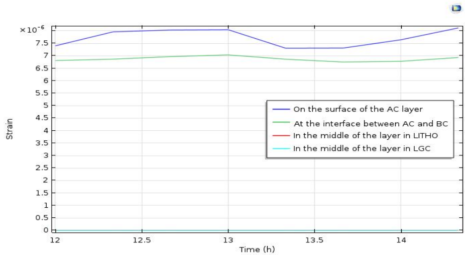
Fig. 9.a Temporal distribution of deformations according to depth in the different layers of NR4 during a rainfall of maximum intensity of 53.06 mm/h.
