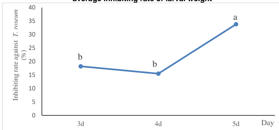
Fig. 2. Insecticidal activity of toxins against L. exigua : A) The average corrected mortality of 3d; B) The average corrected mortality of 4d; C) The average corrected mortality of 5d; D) The average inhibiting rate of larval weight
