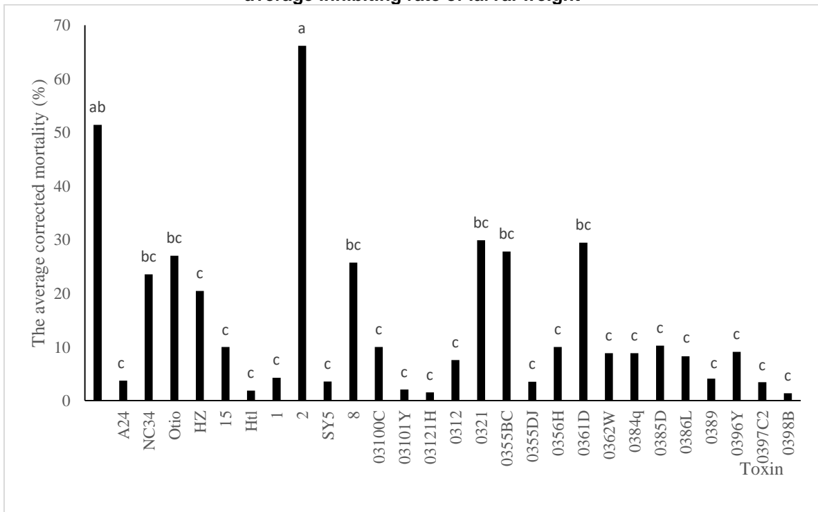
Fig. 1. Insecticidal activity of toxins against P. xylostella : A) The average corrected mortality of 3d; B) The average corrected mortality of 4d; C) The average corrected mortality of 5d; D) The average inhibiting rate of larval weight
