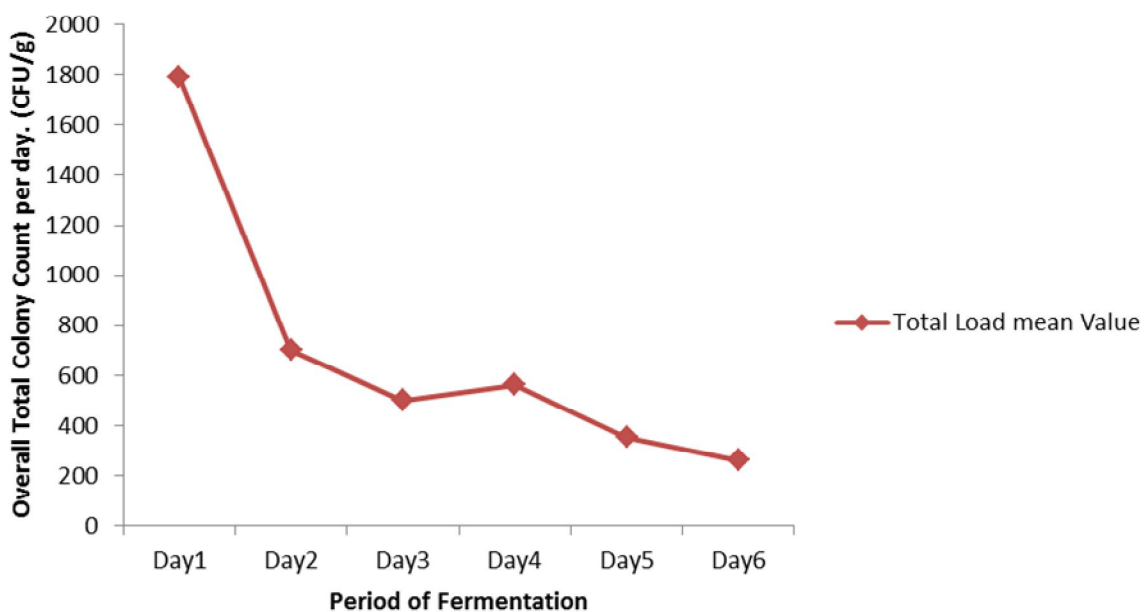
Figure 1: Effect of Solid Fermentation on Daily Total Bacterial Loads
