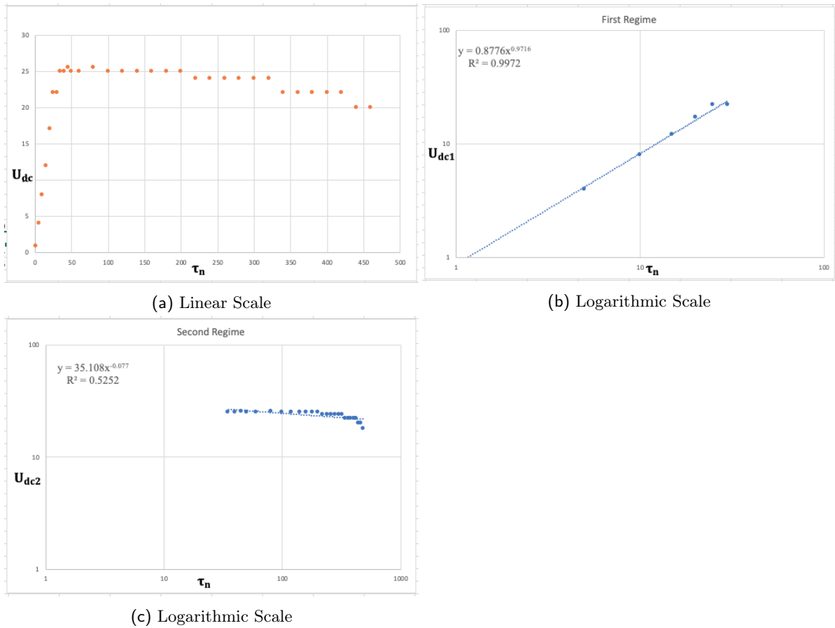
Fig. 4: Propagation speed of the Density current U_{dc} for the different Regimes with respect to time \tau_n for simulations with Re = 50 .
