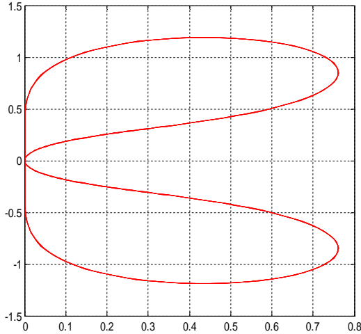
Figure 4. Stability Region for Adams Moulton explicit method for k=4
