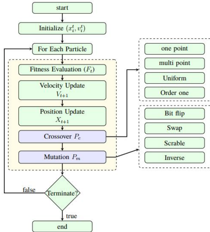
Figure 6: Hybrid Model Flowchart
