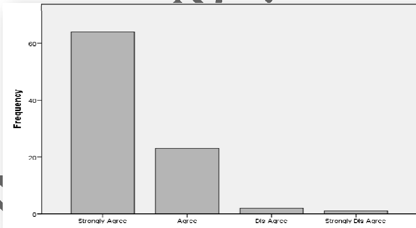
Figure 2 : Language Motivation
