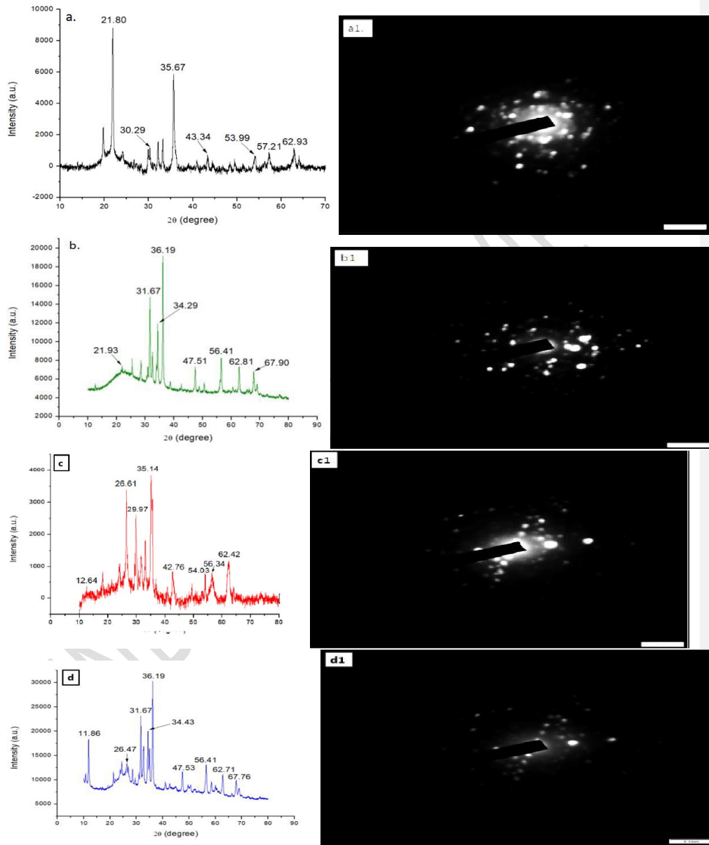
Fig. 2: XRD spectrum of a. mNs – Iron oxide nanocomposite, b. mNs – Zinc oxide nanocomposite, c. rGO – Iron oxide nanocomposite, d. rGO – Zinc oxide nanocomposite. and Selected Area Electron Diffraction (SAED) micrographs of a1. mNs – Iron oxide
