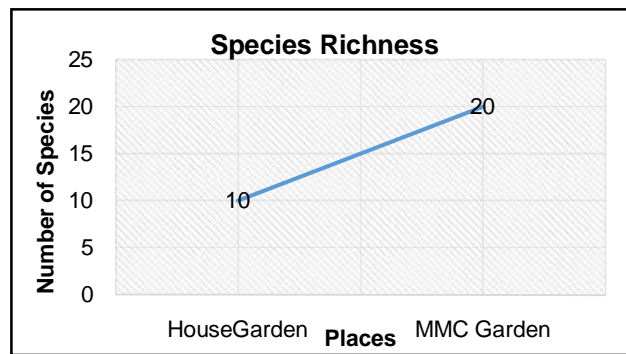
Fig-2: Species Richness on both study areas.
