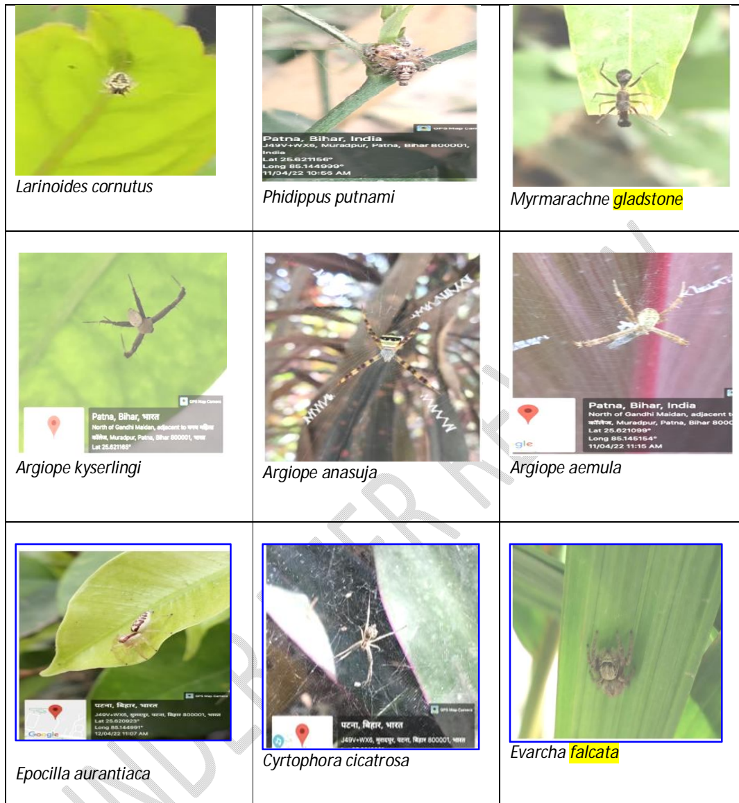
Images- 2 : Different species of spiders investigated in two distinct study areas of Patna (India): Magadh Mahila College Campus garden and House garden
