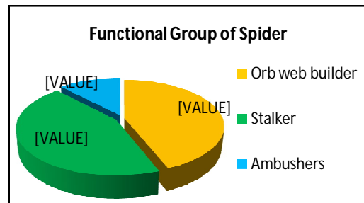
Fig-3: Functional group of spider species.
