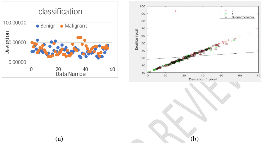
Fig 3 (a) Data before using SVM, (b) data after using SVM
