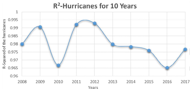
Fig. 7: R-Squared analysis for the years-2008-2017.
