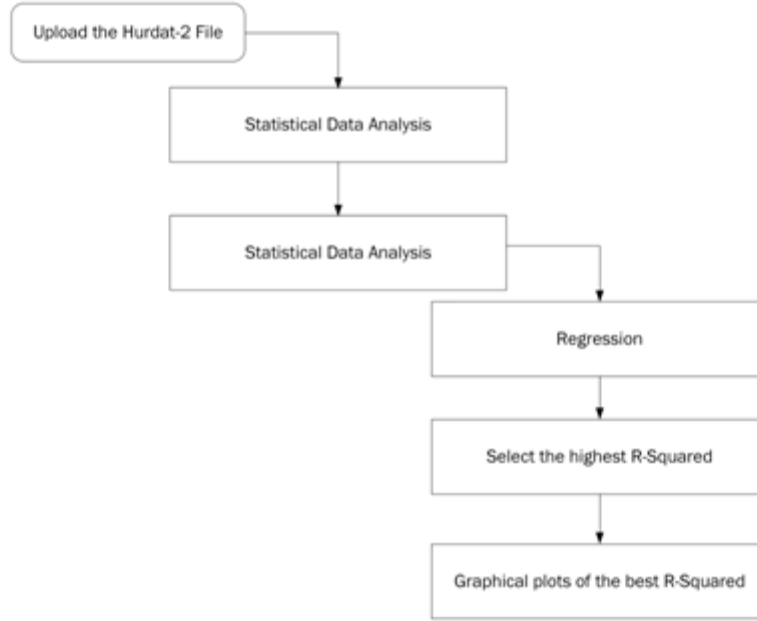
Fig. 2: Proposed Statistical Analysis Model for HURDAT2 Dataset
