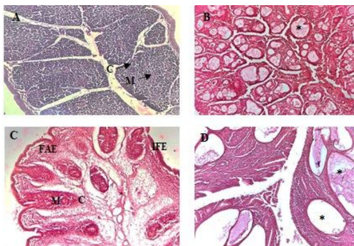
Fig 2 Histological changes in the bursae of fabricius in SPF Birds, A) control, B) BLS+4 at 45X, C) BLS+4 at 100X D) BLS+5 at 100X; IFE: interfollicular epithelium; FAE: follicle-associated epithelium; M: lymphoid follicle medulla; C: lymphoid follicle cortex; Asterisks (*) specify large mucoid cysts in the lymphoid follicles.
