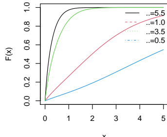
Fig 1c: cdf of CJ distribution
