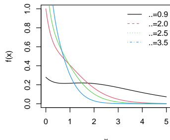
Fig 1a: pdf of CJ distribution
