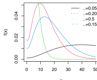
Fig 1b: pdf of CJ distribution
