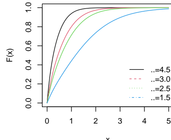
Fig 1d: cdf of CJ distribution
