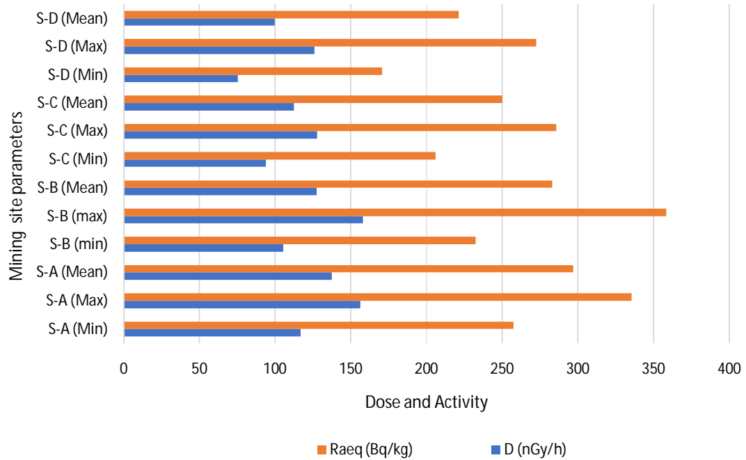
Fig. 3. Gamma Absorbed dose rate and Radium Equivalent Activity.
