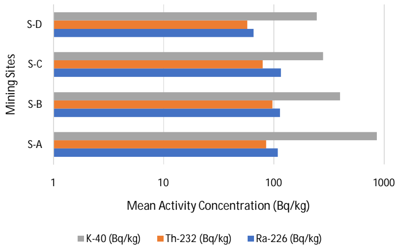
Figure 2: Mean activity concentration of the individual mining sites.
