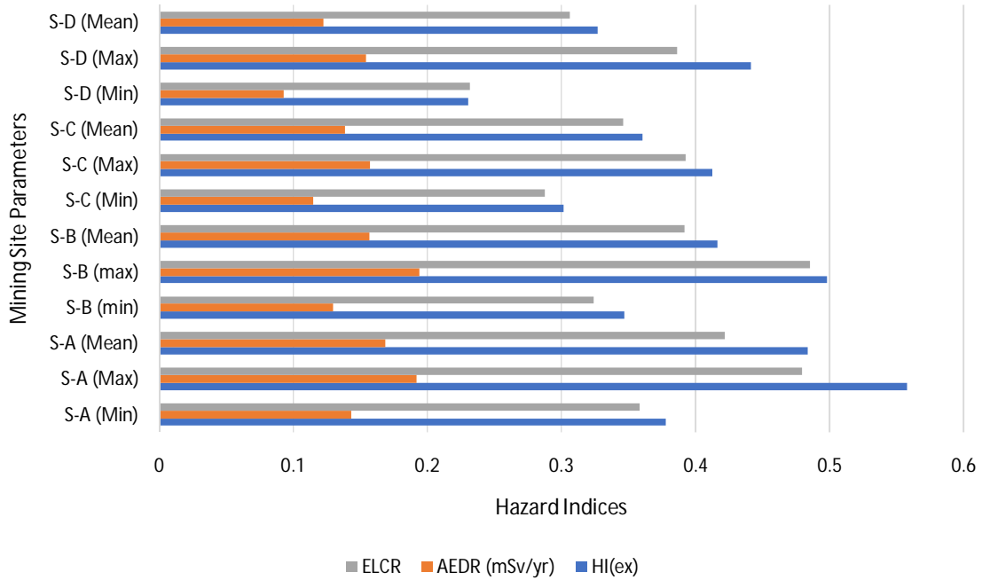
Fig. 4. Excessive Life Cancer Risk, Annual Effective Dose Rate and External Hazard Index.
