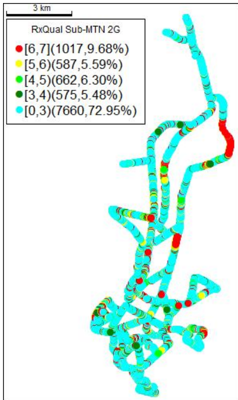
Figure 6: Quality plots of RxQual for MTN Network
