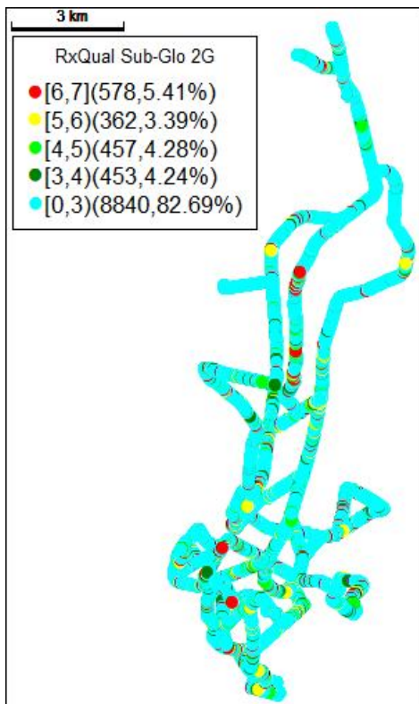
Figure 9: Quality plots of RxQual for Globacom Network
