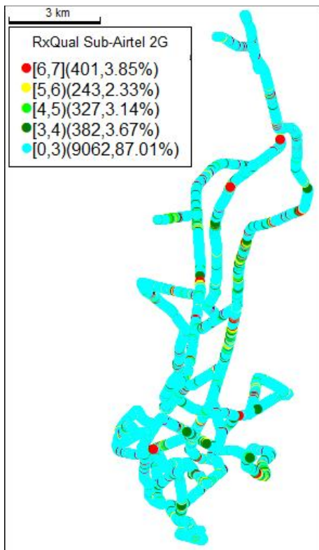
Figure 8: Quality plots of RxQual for Airtel Network
