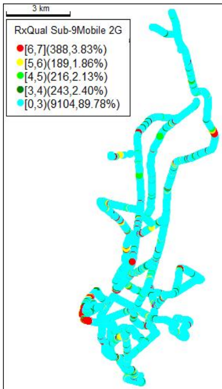
Figure 7: Quality plots of RxQual for 9mobile Network
