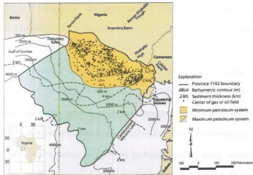
Figure 1 Index map of Nigeria and Cameroon. Map of the Niger Delta showing Province outline (maximum petroleum system); bounding structural features; minimum petroleum system as defined by oil and gas field center points (data from Petroconsultants, 1995a); 200, 1000, 2000, 3000, and 4000 m bathymetric contours and 2 and 4 km sediment thickness.
