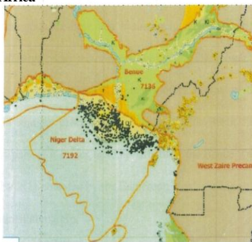
Fig 2 : Geologic map of the Niger Delta and the Benue trough, and the oil fields in the region.
