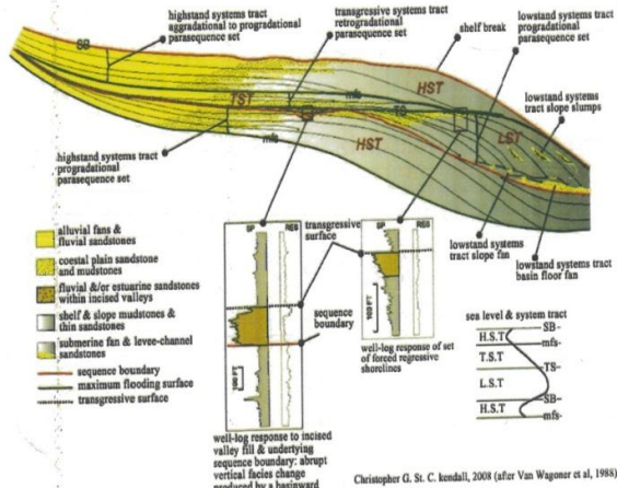
Fig 3: Sea level highstand and lowstand mapped on a crosssection of the basin
