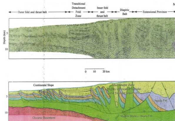
Fig 4: Tectonic Structures drawn over a seismic profile of the Niger Delta Basin
