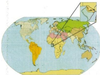
Fig 1 : The Niger Delta Basin is located in the Gulf of Guinea on the west coast of Africa
