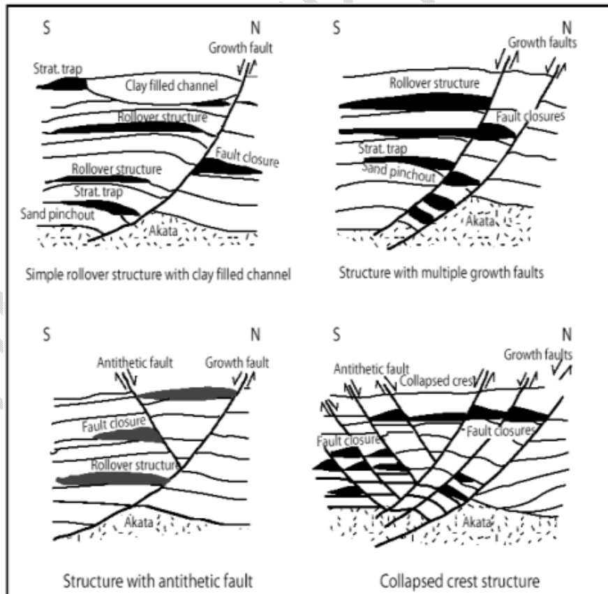
Fig. 3: Schematic Indications of the structural styles and hydrocarbon trapping mechanism in the Niger Delta (Doust and Omatsola, 1990).
