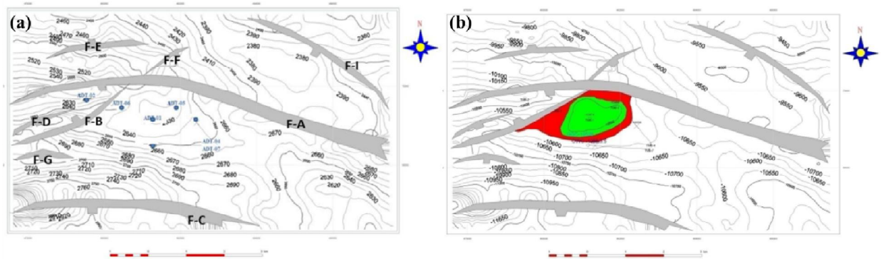
Fig. 15: (a) Sand E Time-Structure Map (b) Sand E Depth-Structure Map
