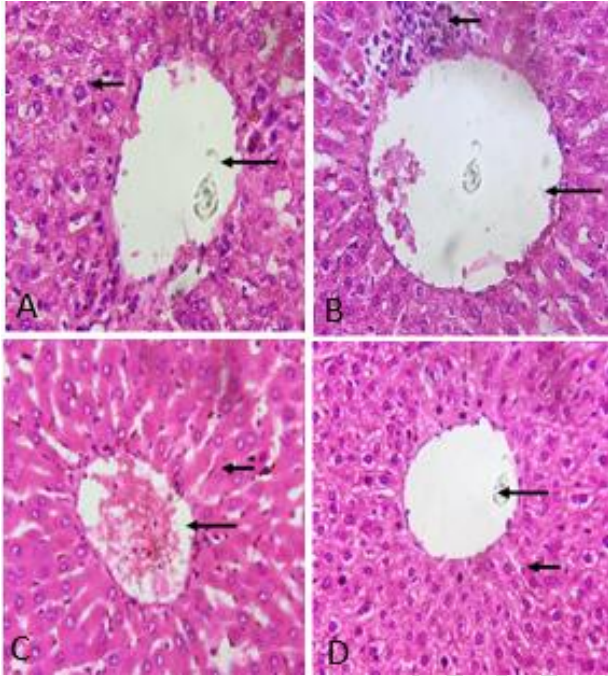
Fig.1 : Histopathological slides
