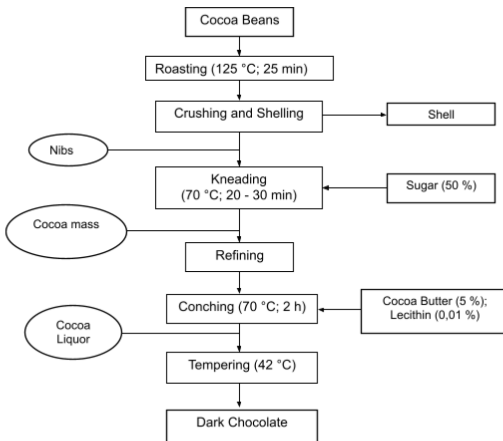
Fig. 4. The manufacturing process of cocoa bean products
