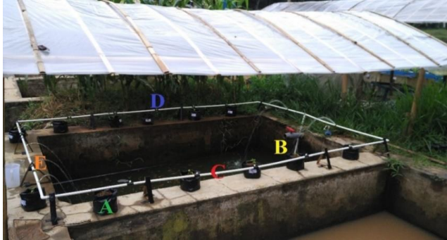
Figure 1. Aquaponics design (A: polybag (Plant), B: pump, C: Parallon, D: faucet/emitter, E: wood bracket)
