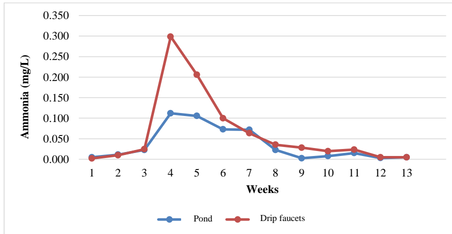
Figure 2. Ammonia graph levels during the study
