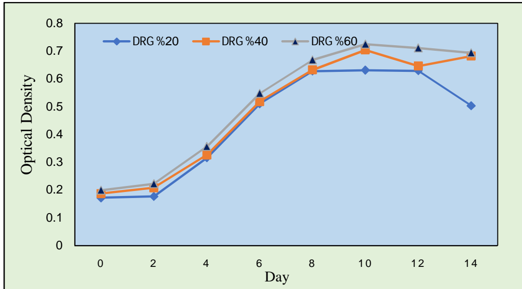
Fig.1. Mean values of optical density of media contained Spirulina platensis
