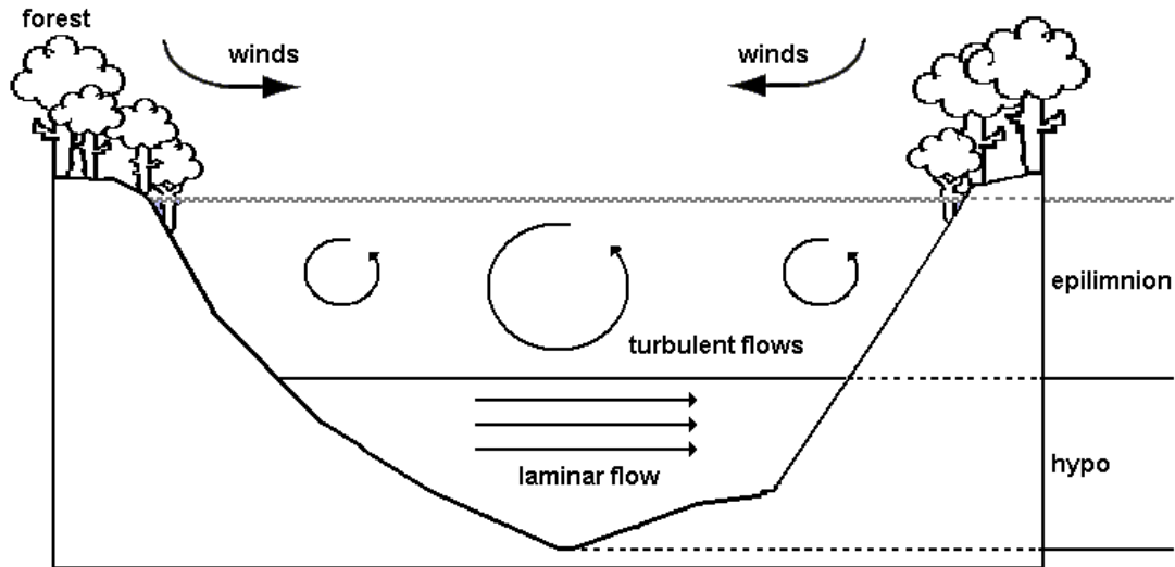
Figure 4: Laminar flow model to Tupé Lake (Central Amazonia, Brazil).
