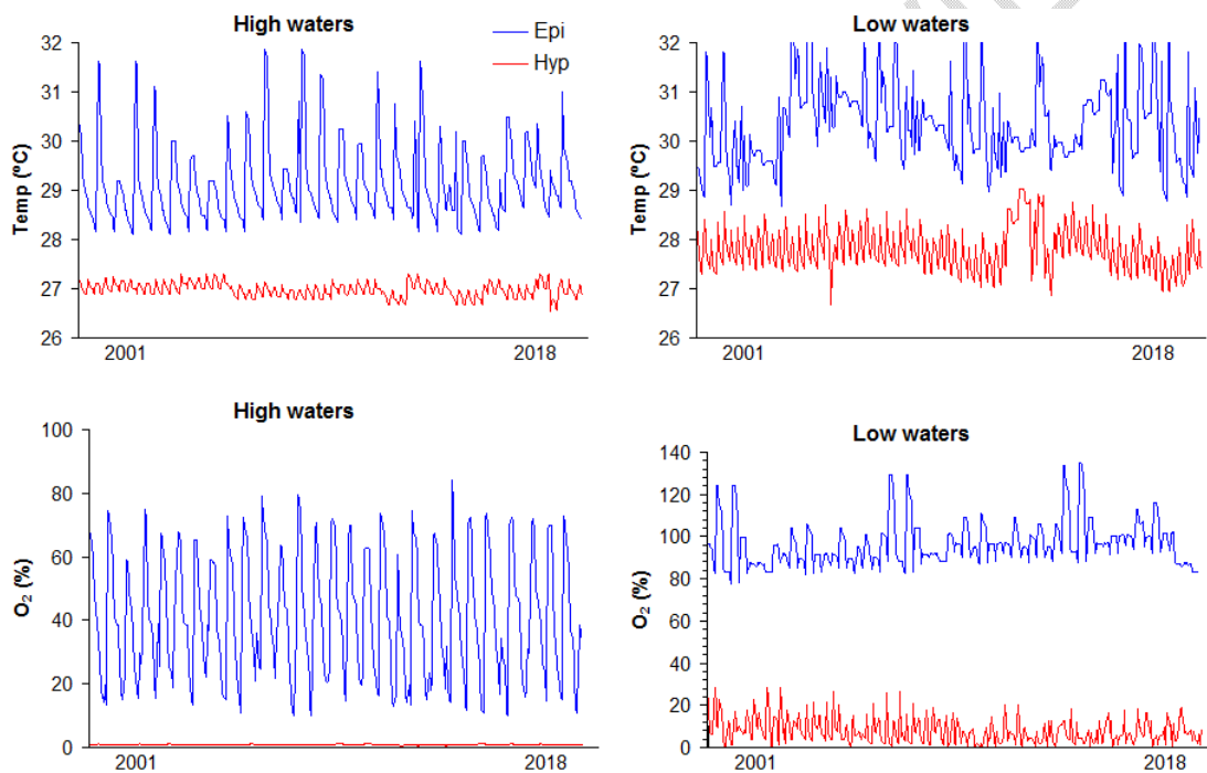
Figure 2: Spatial-temporal variation (2001 - 2018) of temperature (°C) and oxygen saturation (%) for the hydrological year in Tupé Lake, Negro River basin - Amazonas. (N= 2415).
