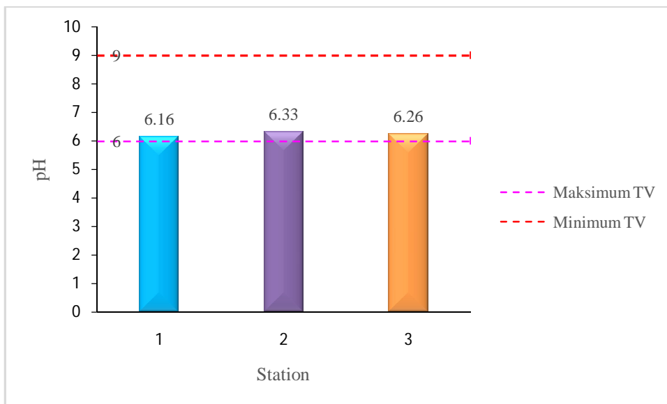
Fig. 9. Average pH of Padjadjaran Retention basin Waters During February to March 2022
