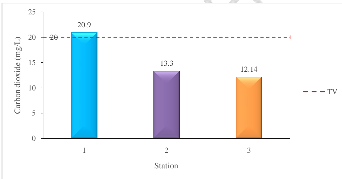
Fig. 8. Average Carbon dioxide of Padjadjaran Retention basin Waters During February to March 2022
