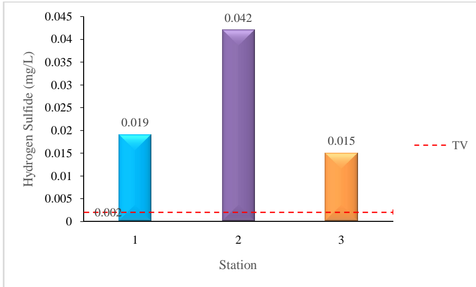
Fig. 12. Average H_2S of Padjadjaran Retention basin waters During February to March 2022
