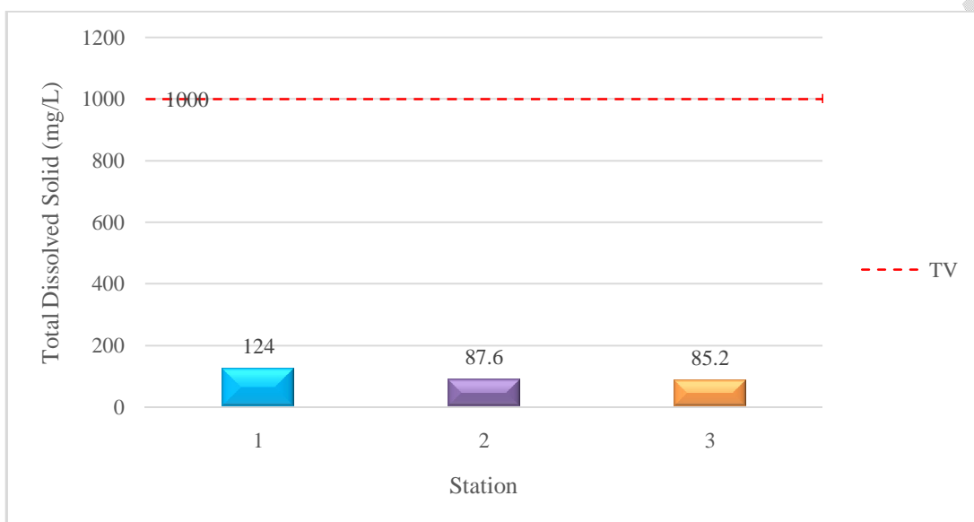
Fig. 5. Average Total Dissolved Solid of Padjadjaran Retention basin Waters During February to March 2022
