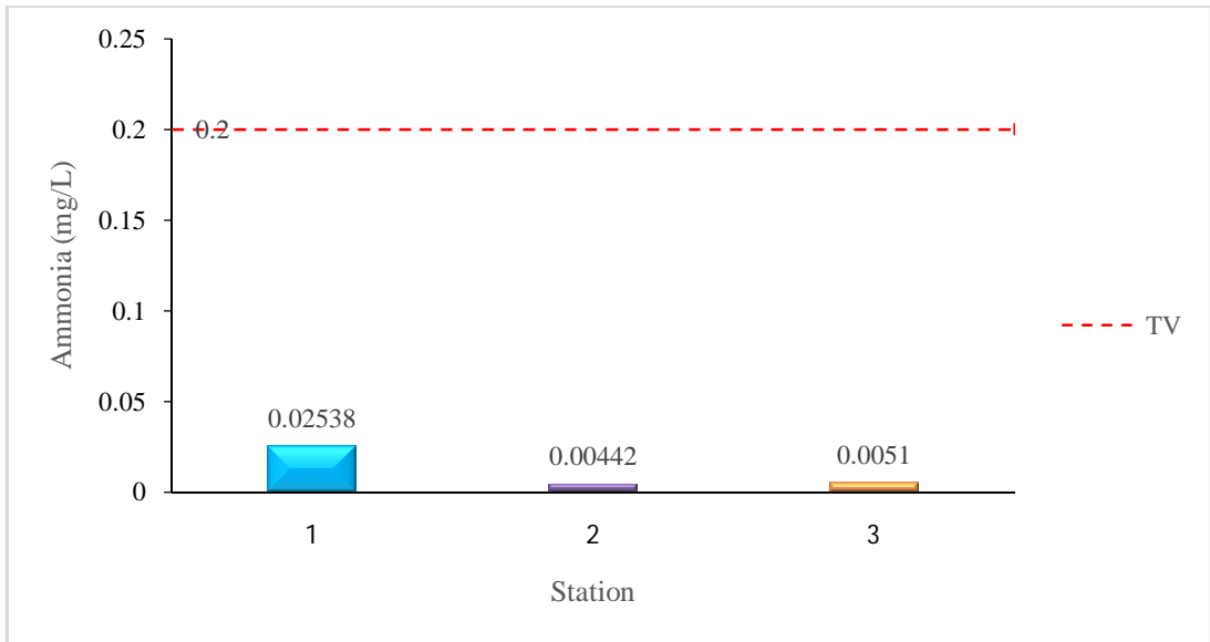
Fig. 10. Average NH 3 of Padjadjaran Retention basin Waters During February to March 2022
