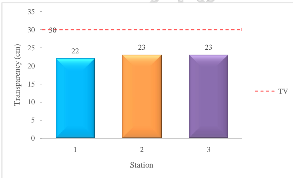
Fig. 4. Average Transparency of Padjadjaran Retention basin Waters During February to March 2022
