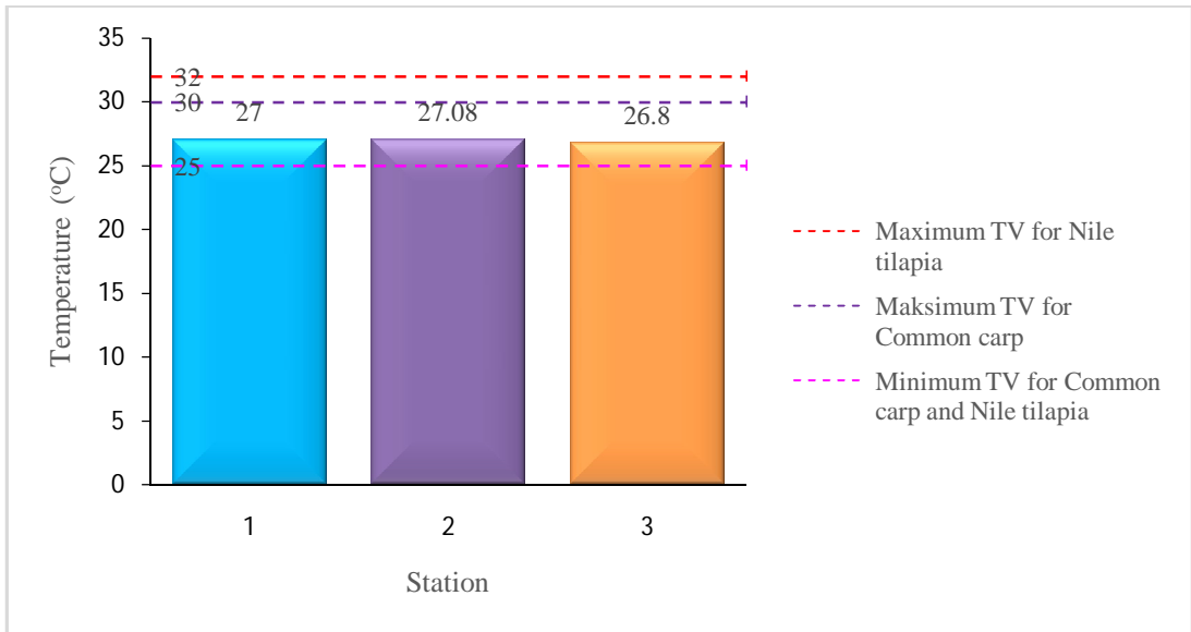
Fig. 3. Average Temperature of Retention basin Padjadjaran Waters During February to March 2022
