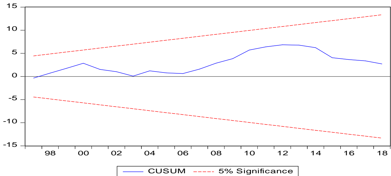
Figure 1a CUSUM
