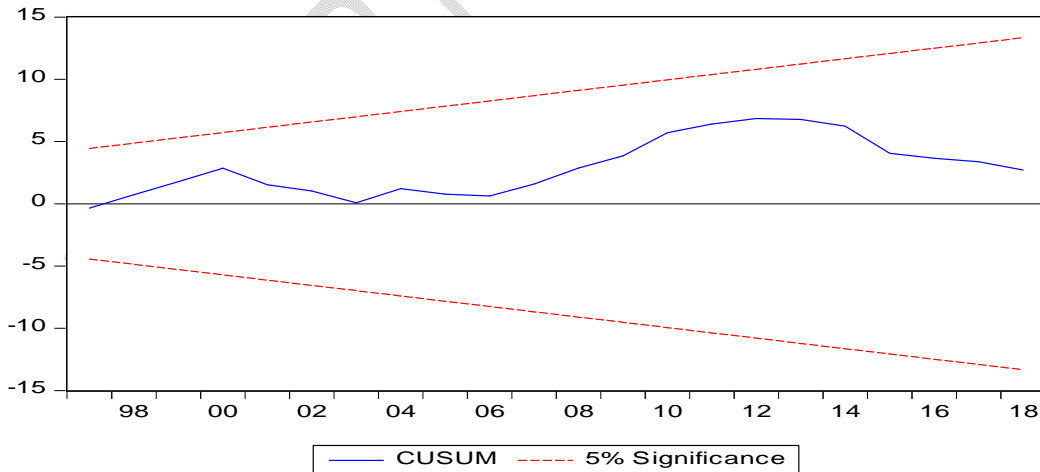
Figure 1a CUSUM
