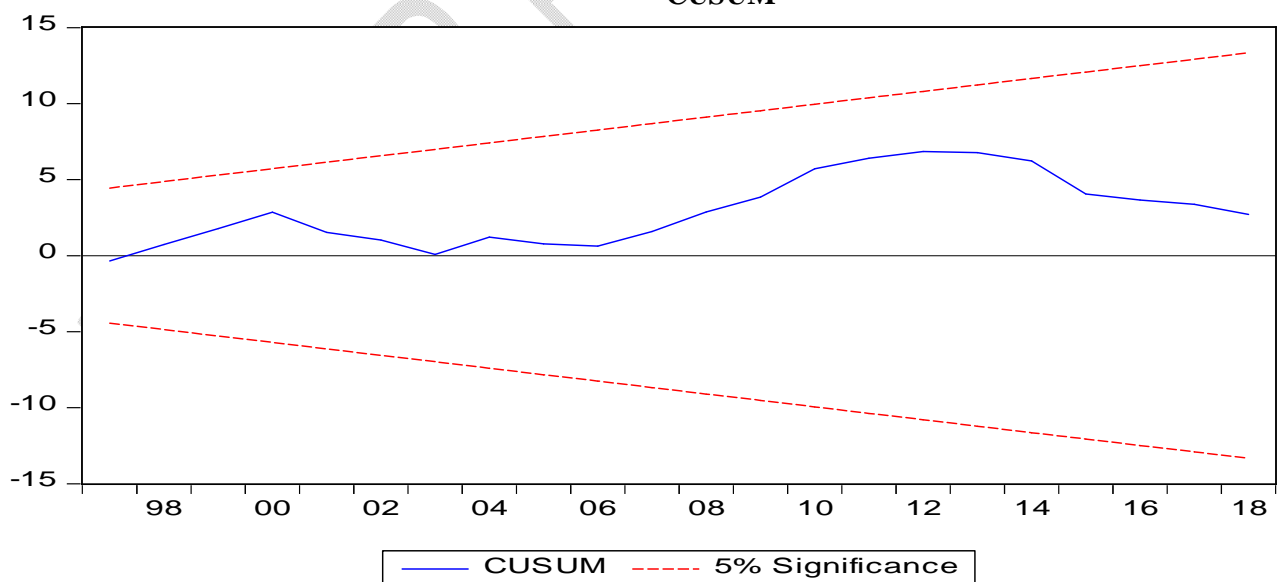
Figure 1a CUSUM
