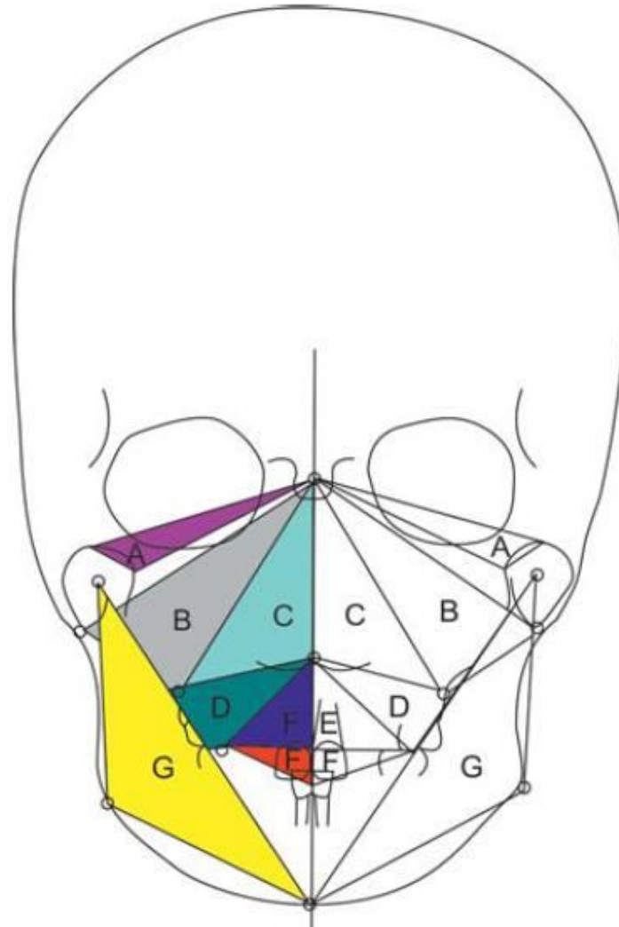
Figure 3. Hewitt's Analysis.
