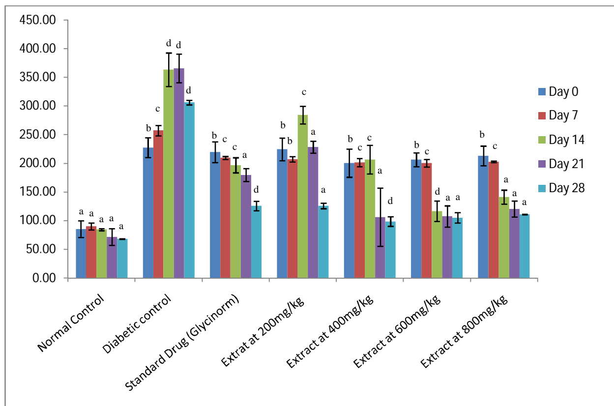
Fig 2: Effects of Hunteriaumbellata methanolic seed extracts on blood glucose levels (mg/dl) Values are the mean \pm SD, n=5. Values in the same column bearing the same letter of the letters are not significantly different ( P > 0.05 ) from each other.
