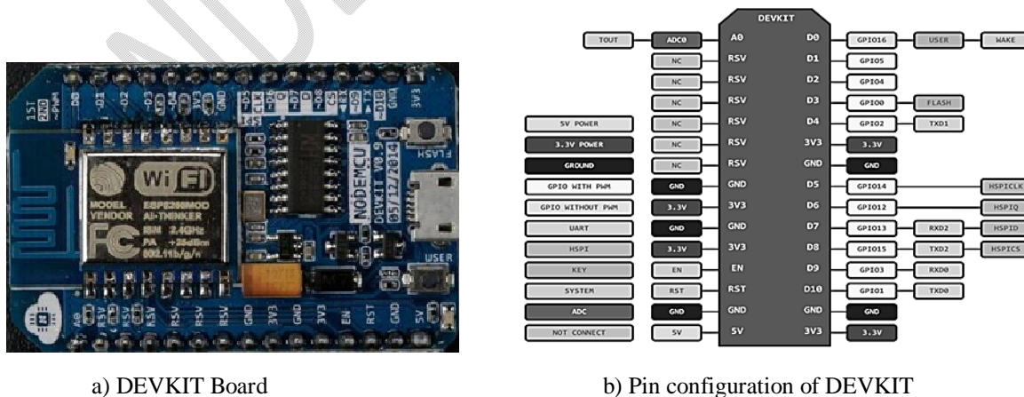
Fig. 4. Node Microcontroller Unit DEVKIT Board and pin configuration [9]
