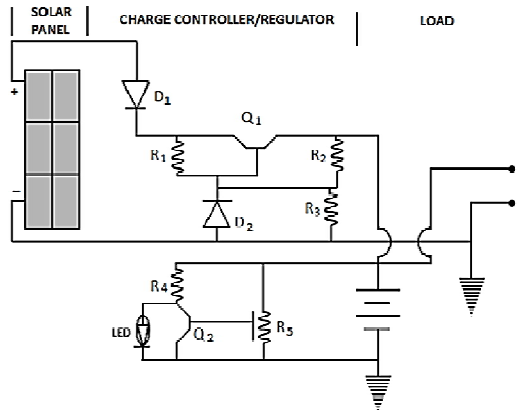
Fig. 3. Circuit diagram of the solar power supply [8]
