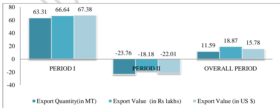
Figure 2: Compound Growth Rate of Export quantity and Export Value of Maize
