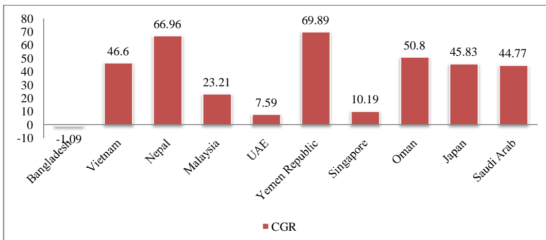
Figure 3: Compound Growth Rate of Maize exported from India in quantity during the study period
