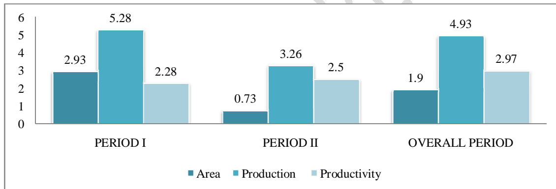
Figure 1: Compound Growth Rate of Area, Production and Productivity of Maize in India During overall study period (1999-2000 to 2018-2019) area, production and productivity recorded positive and significant growth rate of 1.90 per cent, 4.93 per cent and 2.97 per cent at one per cent level of significance. The results were in close association with findings of Ayalew & Sekar (2016), Dhakre & Sharma (2010), Patil et al. (2018) and Swamy et al. (2019) [8].
