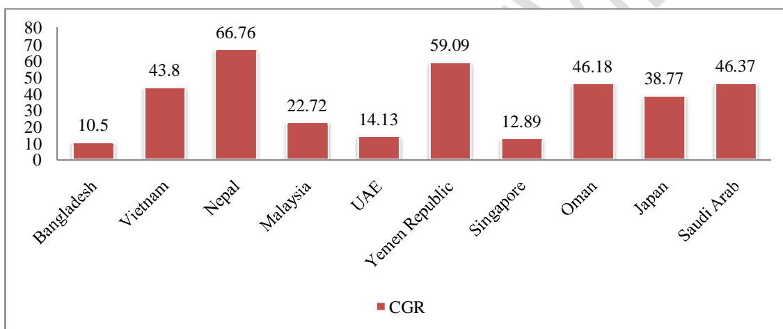
Figure 4: Compound Growth Rate of Maize exported from India in value measured in Indian Rupees during the study period
