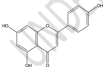
Apigenin
