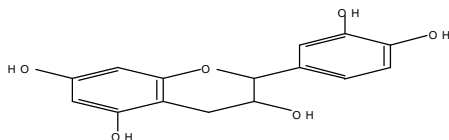
Catechin
