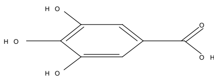
Gallic acid
