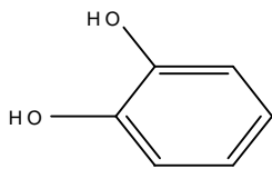
Pyrocatechol
