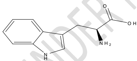
Tryptophan
