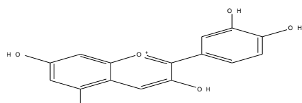
Cyanidin
