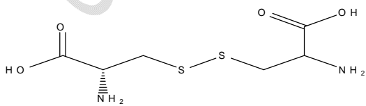
Cystine
