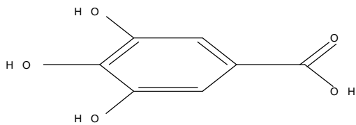
Gallic acid
