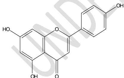
Apigenin
