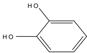
Pyrocatechol
