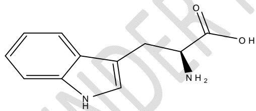
Tryptophan
