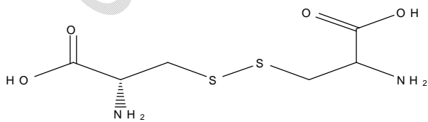
Cystine
