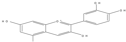
OH Cyanidin
