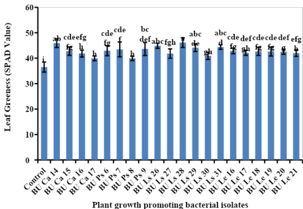
Fig. 2. Influence of plant growth promoting bacteria on leaf greenness (SPAD Value) of rice (Error bar indicates standard deviation of mean)
