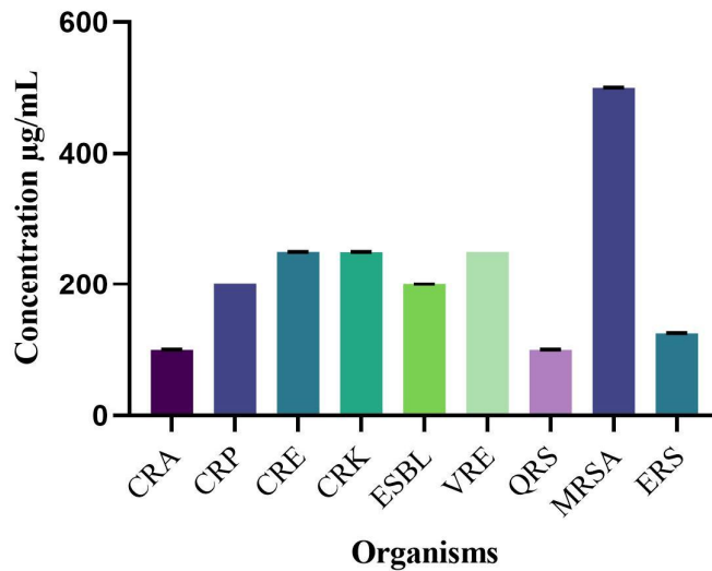
Figure 4: Graph representing the minimum inhibitory concentration of Cymbopogon martini essential oil against selected drug-resistant strains. CRA- Carbapenem Resistant Acinetobacter species , CRP- Carbapenem Resistant Pseudomonas aeruginosa , CRE- Carbapenem Resistant E. coli , CRK- Carbapenem Resistant Klebsiella pneumoniae , ESBL- Extended Spectrum beta lactamase E. coli , VRE- Vancomycin resistant Enterococci , QRS- Quinolone resistant Salmonella , MRSA- Methicillin resistant Staphylococcus aureus , ERS- Erythromycin resistant Streptococci.
