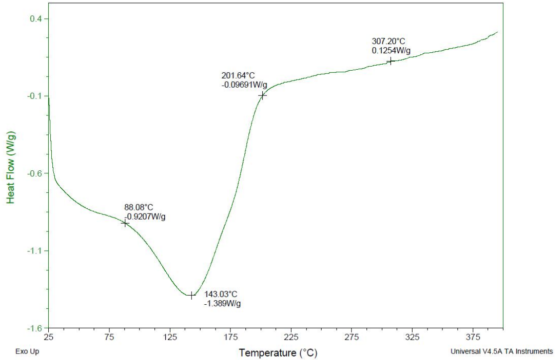
Figure 3: Thermogram representing differential scanning calorimetric analysis of Cymbopogon martinii essential oil at constantly increasing temperatures.
