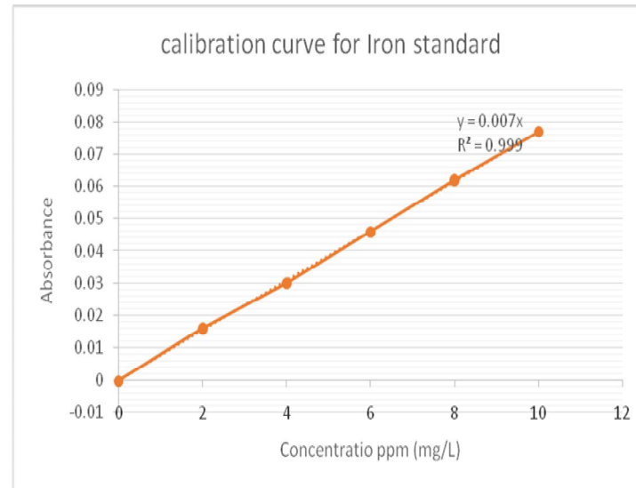
Figure 1.0 Calibration curve for Iron standard
