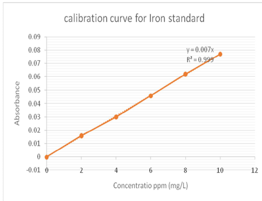
Figure 1.0 Calibration curve for Iron standard
