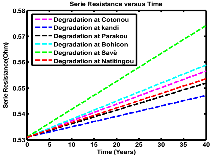
Fig. 11. Series resistance degradation
