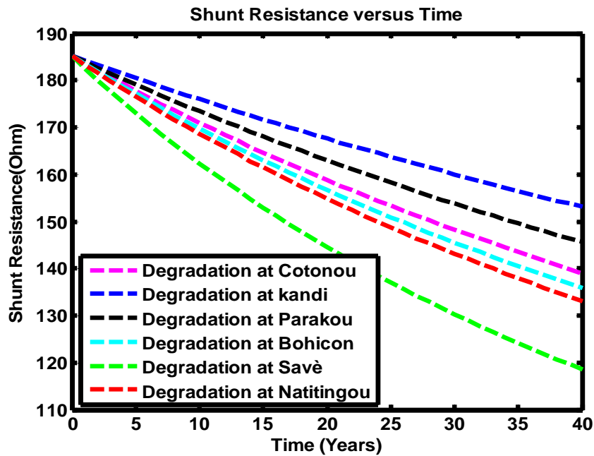
Fig. 10. Shunt resistance degradation
