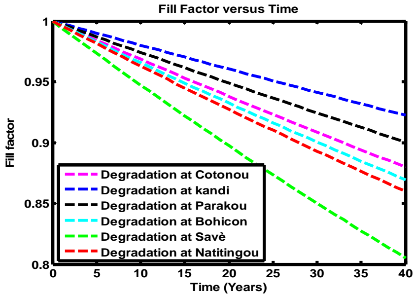
Fig.12. Fill Factor degradation
