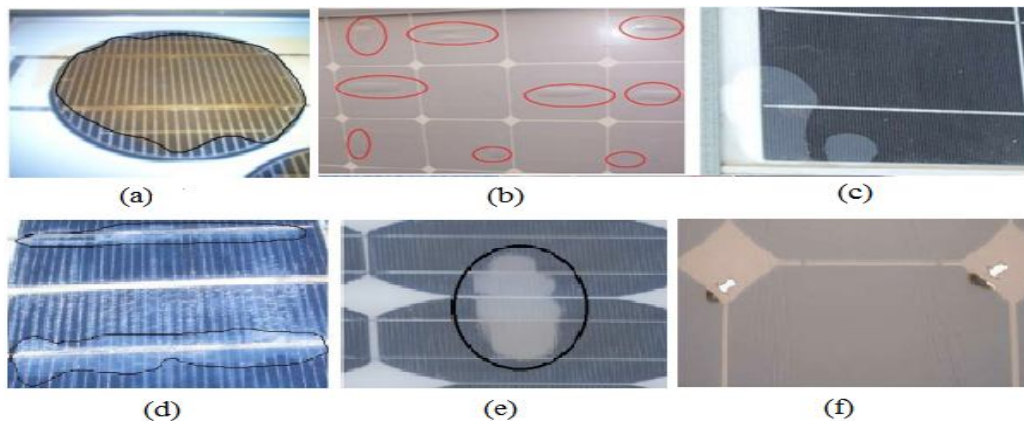
Fig.1: (a) Discoloration of the encapsulant, (b) Bubbles rear face, (c) Bubbles front face, (d) and (e) Delamination of the encapsulant and (f) Hot spot [3, 4, 5, 6].
