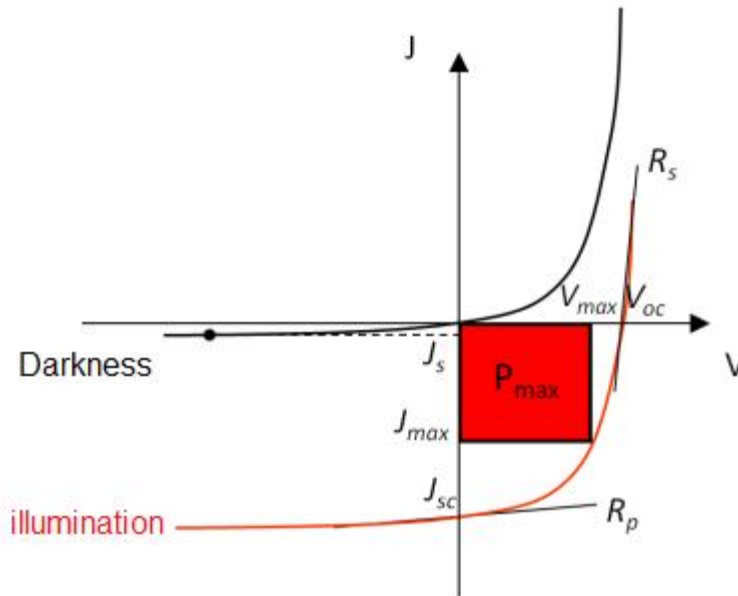
Figure 8: I-V characteristics under darkness and under AM1.5 lighting [50]
