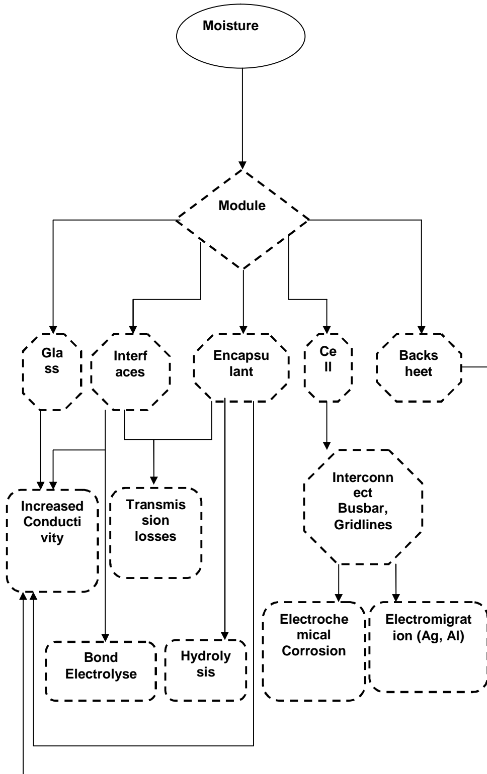
Fig. 6. Effects of moisture and degradation mechanism [47]
