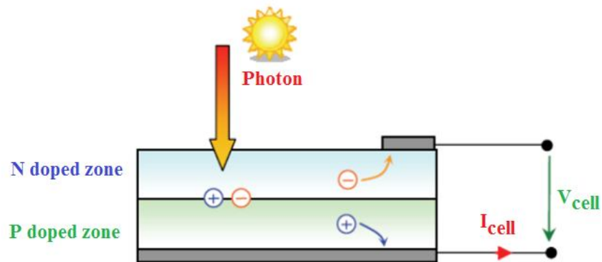
Fig.4. Schematic diagram of photoelectric conversion [3]
